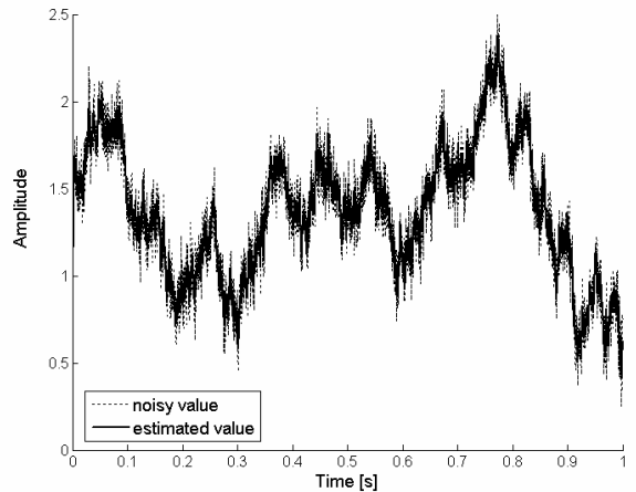
Figure 3. Amplitude estimation.
